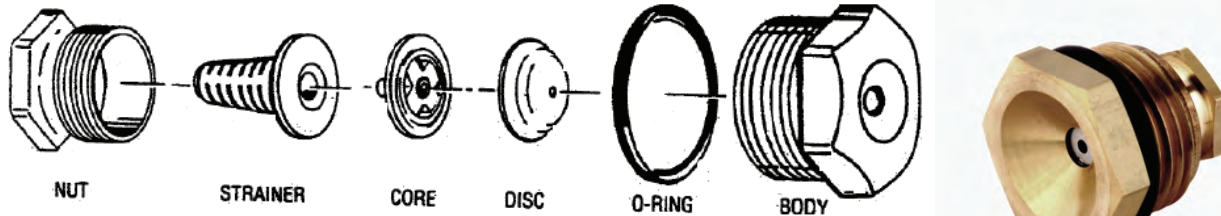
L-W Nozlet Full Cone Spray Nozzle (1 1/16" NPT pipe thread)
