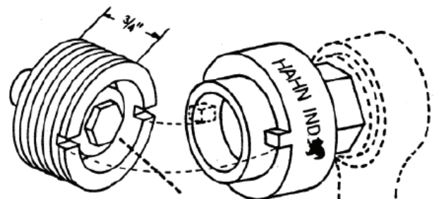
Above - Spraylet adapter (368-00000) with a 1 1/16" outside thread.
