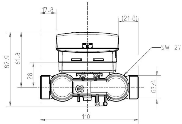
Mounting length 110 mm
