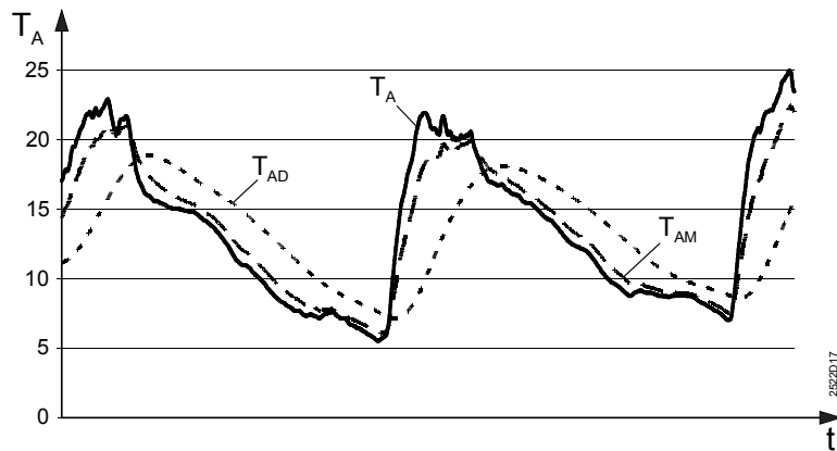
Progression of current, composite and attenuated outside temperature
