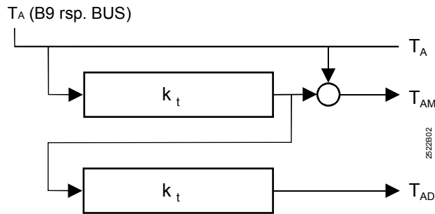
Generation of composite and attenuated outside temperature
