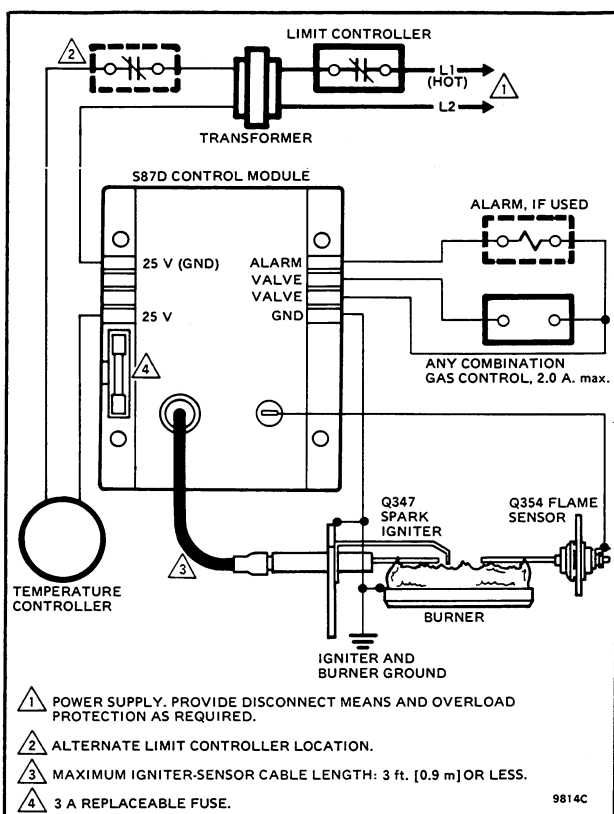
FIG. 5—S87D IN TYPICAL HOOKUP FOR DIRECT SPARK IGNITION HEATING SYSTEM. SEE FIG. 16 FOR SYSTEM SCHEMATIC DIAGRAM.
