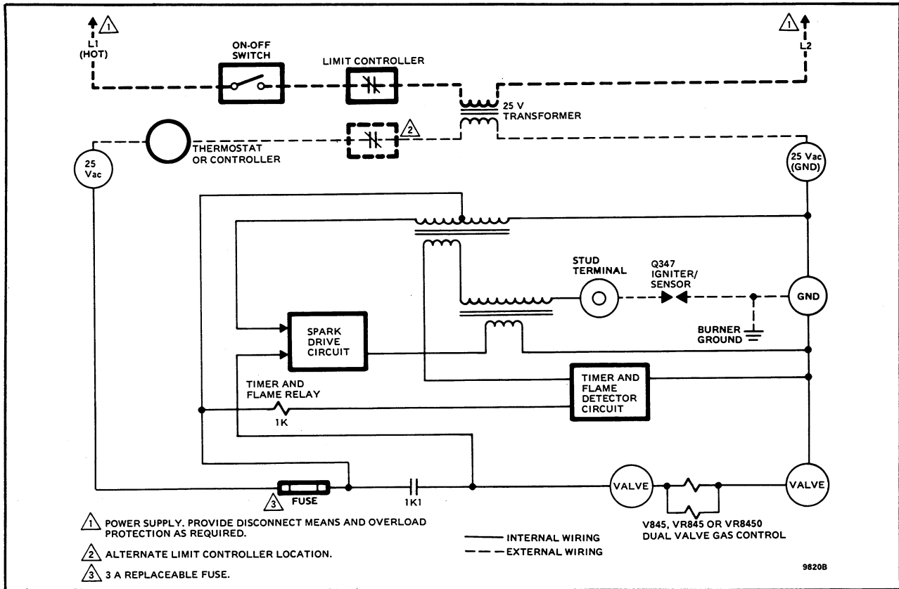
FIG 13—S87A SIMPLIFIED SYSTEM SCHEMATIC.
