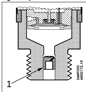
Figure 5: pulse snubber
