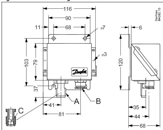
Figure 6: Dimensions diagram
