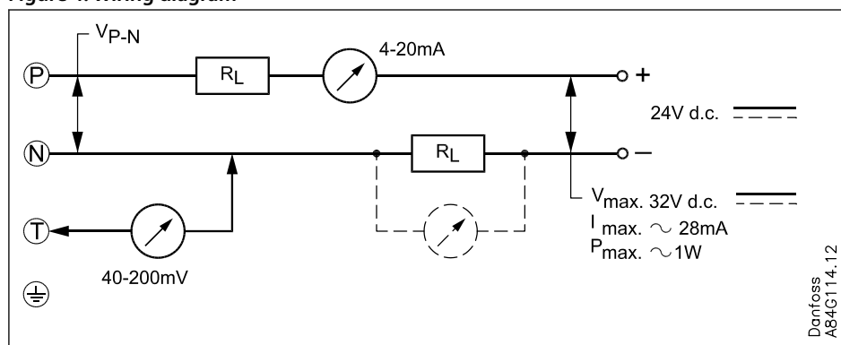
Figure 4: Wiring diagram
